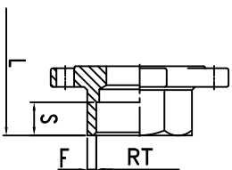
MODEL YK531S Socket Weld End
