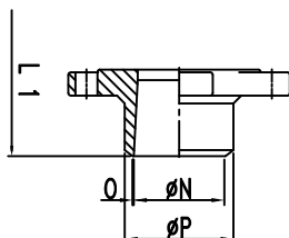
MODEL YK531B Butt Weld End
